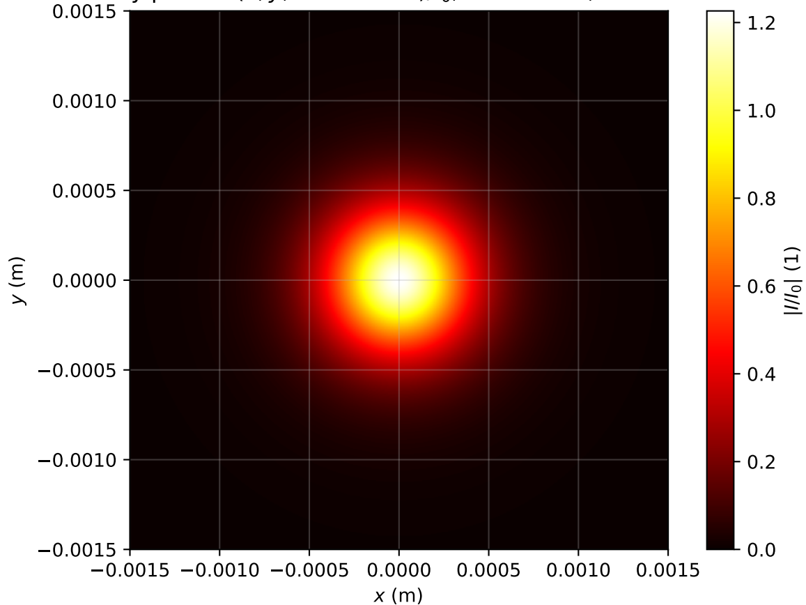
Intensity profile I(x, y, z = 2.468m)/I_0 , P_{in}=0.8P_{cr} , artificial time
